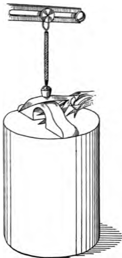
FIG. 33.—Detail of arrangement of auxograph to record variations in thickness of leaf of Messembryanthemum . Leaf in a horizontal position resting on a wooden support cut away below to make place for the younger terminal leaves.
